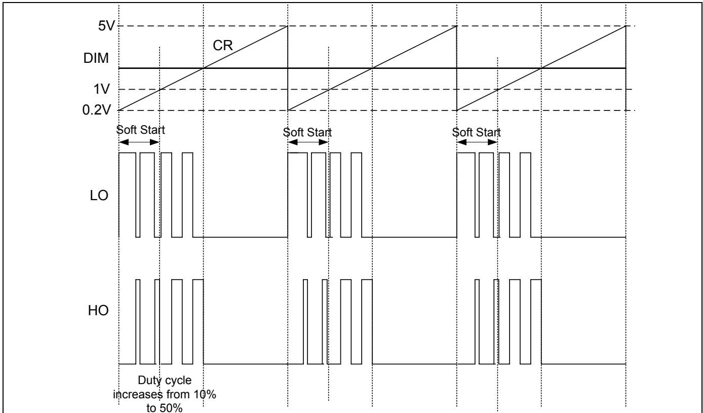
Figure 4: Dimming waveform
